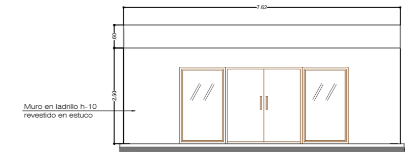
FACHADA PRINCIPAL
